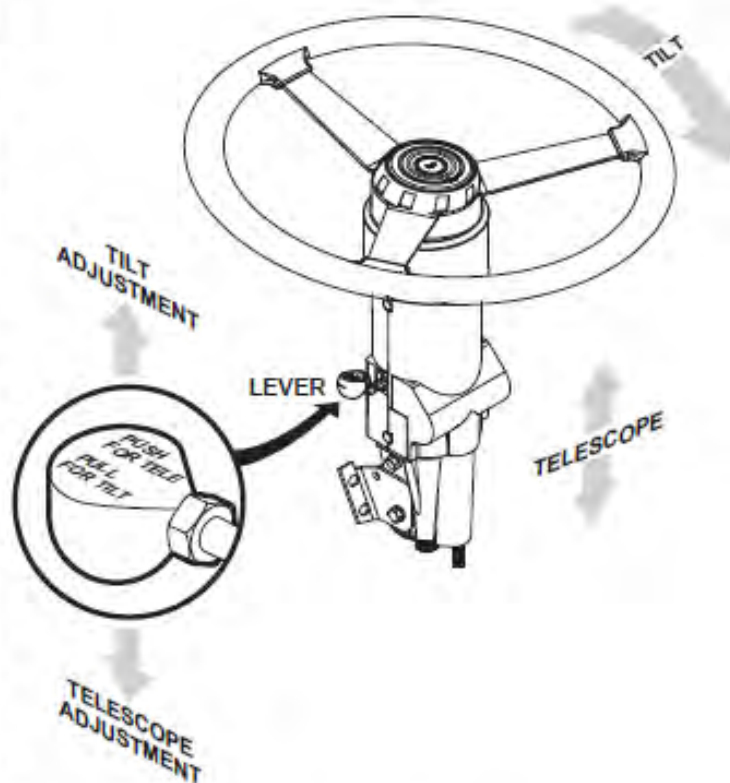
Steering Column Adjustment
