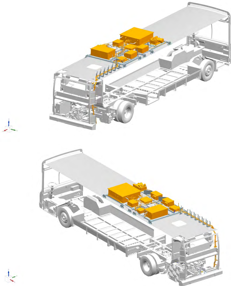
Fig. 1.6. GILLIG Hybrid Electric Bus High Voltage System Layout
