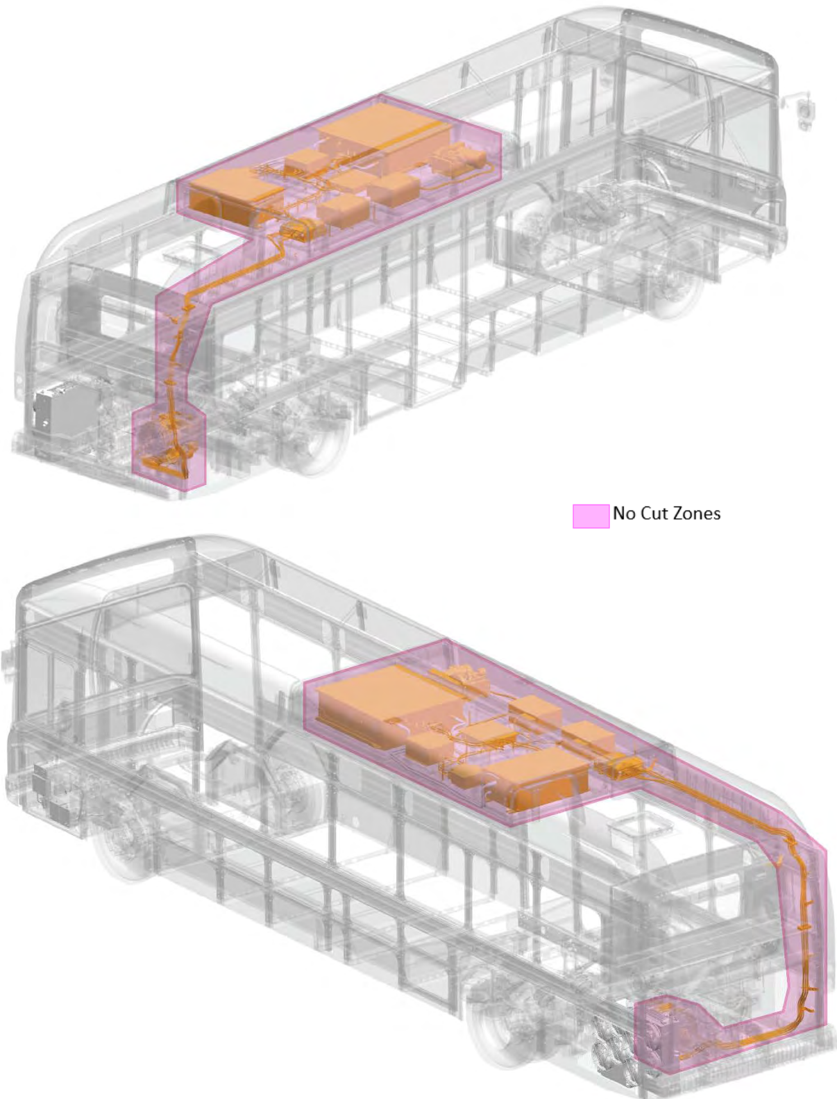
Fig. 4.2 No Cut Zones
