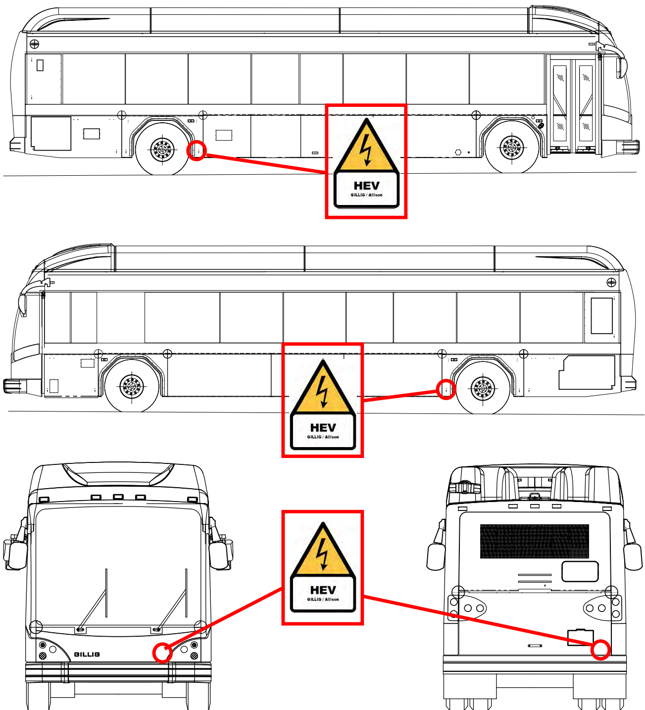
Fig. 1.2. GILLIG Hybrid Electric Vehicle Badging Locations
